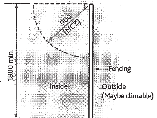
Boundary fence climbable on the outside
