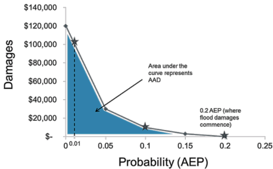
Figure J-15 Loss probability curve
